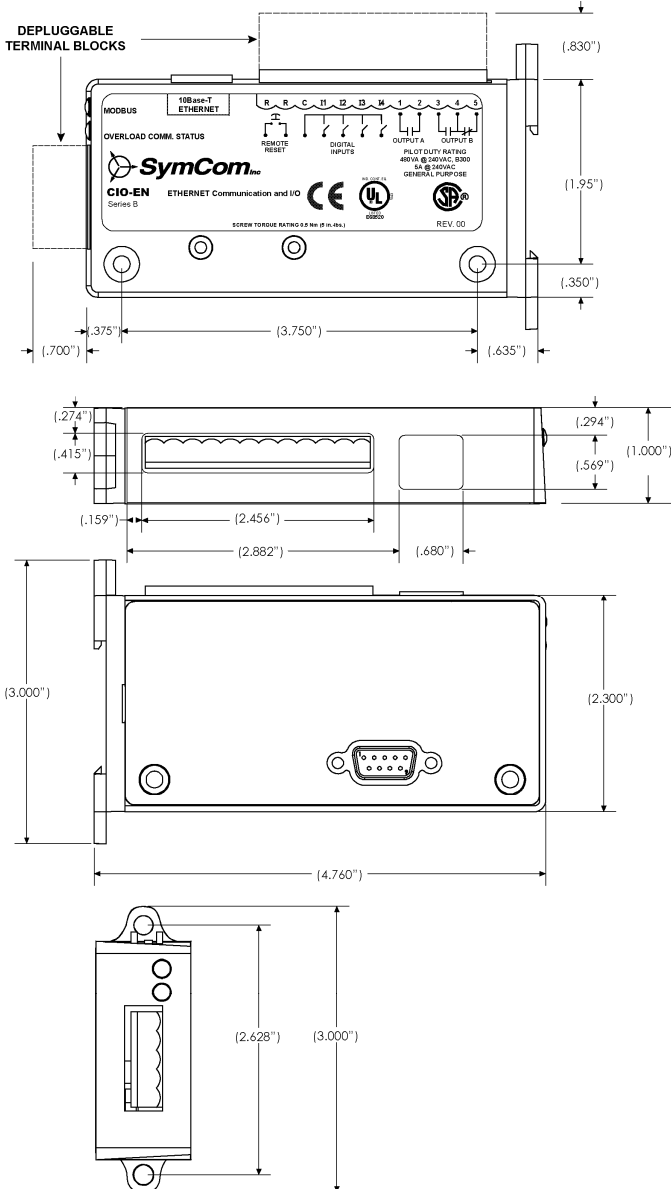
FIGURE 3: Physical Dimensions (CIO-EN)
