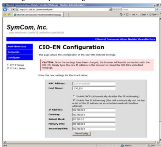
Figure 2: CIO-EN Embedded Webpage
