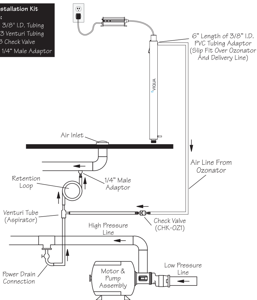
Figure 2 Pressure Differential System
